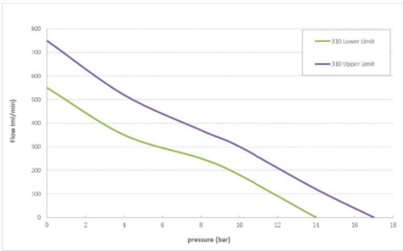
310 Series Curve
