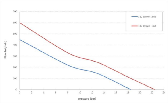
312 Series Curve
